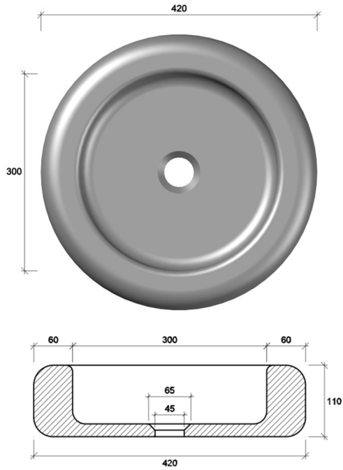
Piece Dimensions
